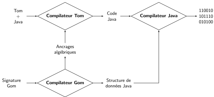
Figure : TomGomCompiler
